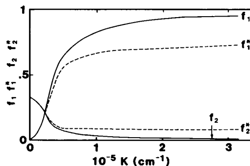
FIGURE 5 Graphic representation of functions f_1(k) and f_2(k) for a rigid rod and f_1^*(k) and f_2^*(k) for a semiflexible rod with \gamma L = 0.49 , L = 1.90 \mu\text{m} , and d = 7.0 \text{ nm} . For details, see Appendix.
